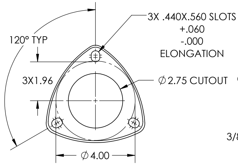
MOUNTING PLATE (MP-132)
